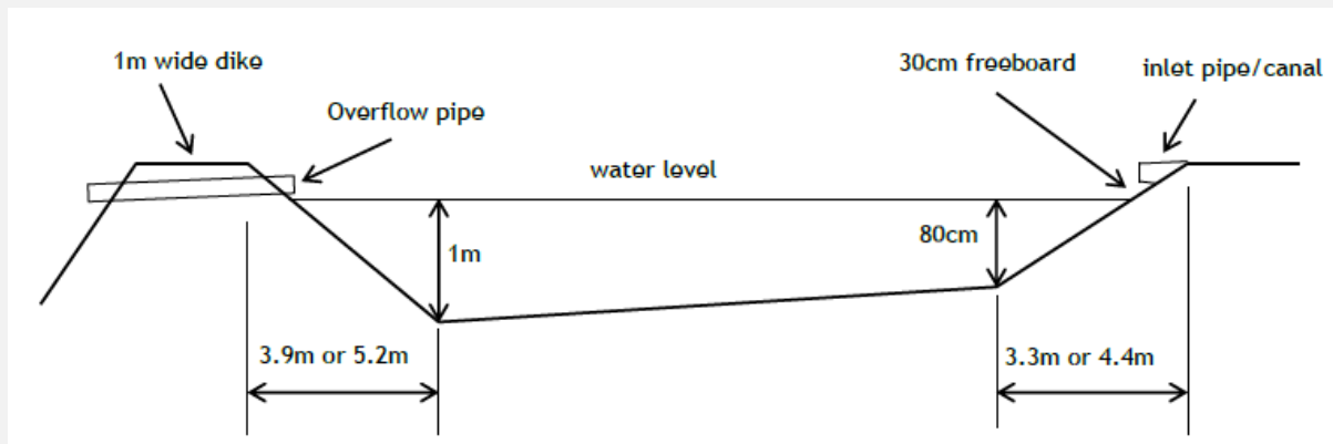
Figure 9 Cross-section of a fish pond (Source: Peacecorps, 2014)
